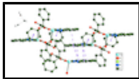
Fig. 2. A packing view of the title compound. C—H... \pi interactions and \pi - \pi stacking interactions are shown as dashed lines.
